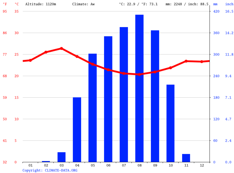
Figure 1. Ombrothermic diagram.
